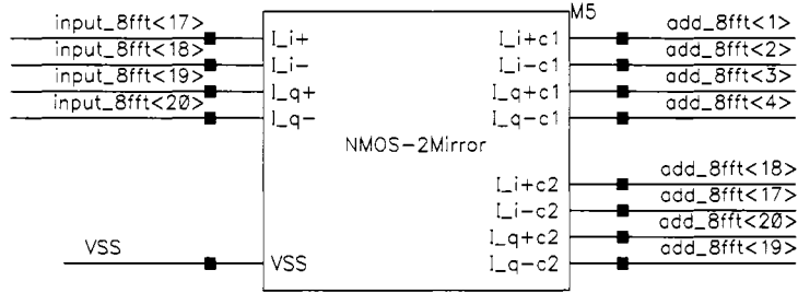
Figure 3.11: First basic block of the lower half part of the 8-FFT stage.
