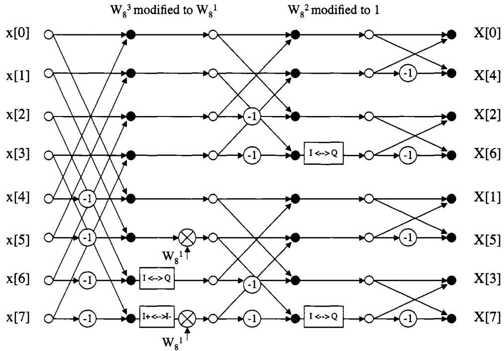
Figure 3.3: Modified Butterfly Diagram for 8-FFT .
