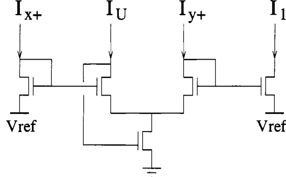
Figure 2.4: Basic block of analog differential multiplier with translinear loop [1].
