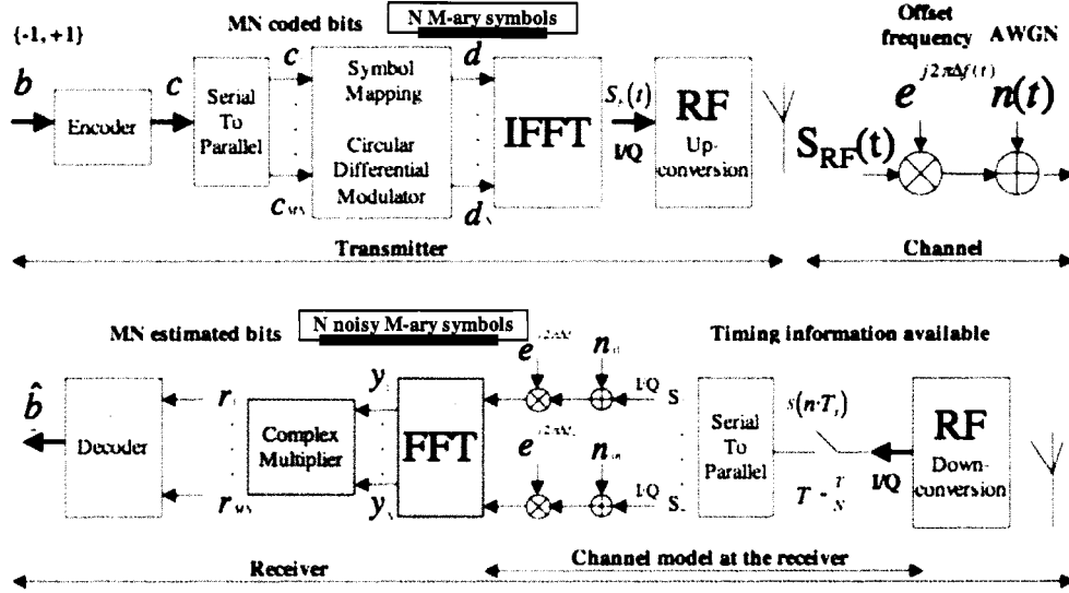
Figure 2.2: OFDM communication system model.
