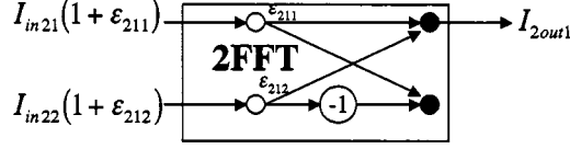
Figure 3.18: Mismatch for the 2-FFT block. Each current mirror has its \varepsilon_{sci} where s indicates the stage, c is either 1 or 2 representing the first or second copy of an input i .
