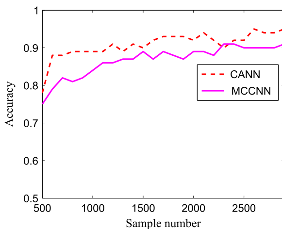
Fig. 5. The impact of training sample number on classification accuracy of CANN and MCCNN.
