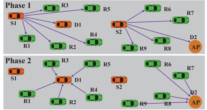
Fig. 1. Two phases of DF cooperative communication with multiple relays in a VANET. In the first phase, the source nodes (e.g., S1 and S2 ) broadcast their information to the corresponding relays (e.g., \{R1, R2, \dots, R9\} ) as well as to their destinations (e.g., D1 and D2 ). Then, these relays can re-transmit the information to the corresponding destinations on orthogonal sub-channels during the second phase.
