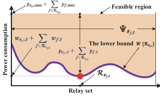
Fig. 2. A sketch of the power consumption bound curve.
