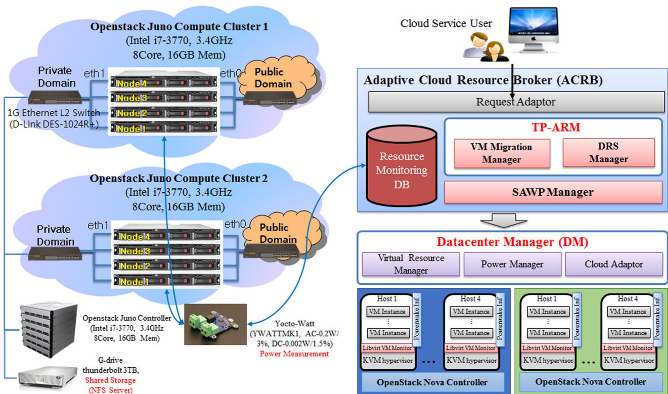
Fig. 6 Experimental Environment
