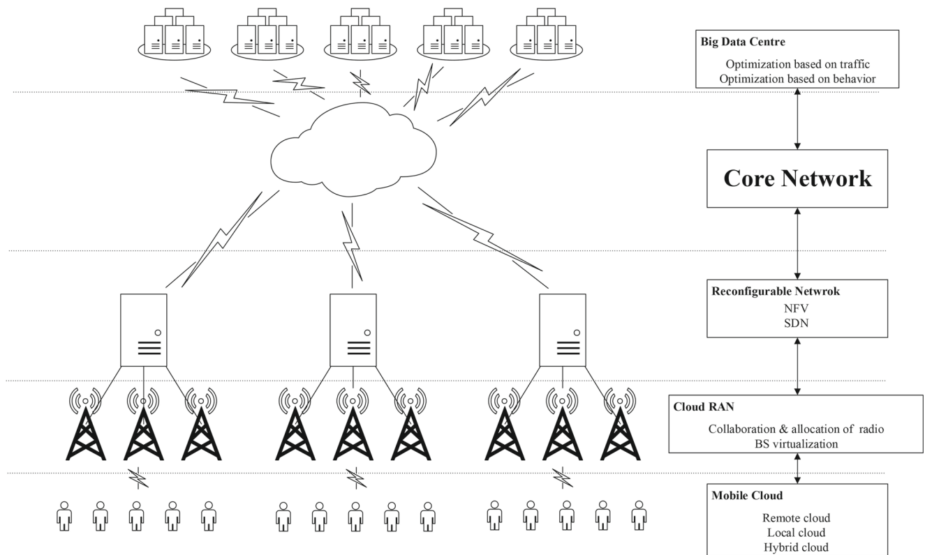
Fig. 1 Cloud-based wireless network architecture
