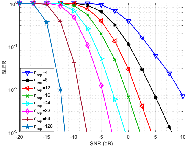
Fig. 8. BLER vs SNR for different repetitions ( n_{rep} ) of PUSCH with TBS of 504 bits in NTN TDL-A channel.
