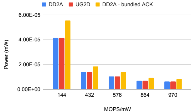
Fig. 11. Power consumption for implementing our solution in a UE with different processor architectures.
