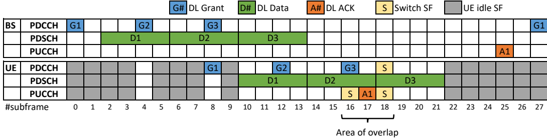
Fig. 4. An illustration of the scheduling conflict with TB overlap using the current-day method. BS: base station; UE: user equipment; PDCCH: physical downlink control channel; PDSCH: physical downlink shared channel; PUCCH: physical uplink control channel; G1, G2, and G3 are the downlink grants scheduling the downlink data D1, D2, and D3, respectively. D1, D2, and D3 are each repeated four times and therefore span four subframes each. A1 is the acknowledgment subframe of D1. S represents a switching subframe. Subframes shaded grey represent occasions where the UE is neither transmitting nor receiving, and therefore contributing to a reduction of the throughput. The area of overlap represents the subframes where the HD-FDD UE is erroneously expected to transmit on PUCCH and simultaneously receive on PDCCH and PDSCH, which renders this scheduling scenario inoperable.
