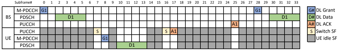
Fig. 3. Timing diagram for downlink operation in NTN. BS: base station; UE: user equipment; M-PDCCH: machine-type communication physical downlink control channel; PDSCH: physical downlink shared channel; PUCCH: physical uplink control channel. G1 is the downlink grant scheduling the downlink data D1. D1 is repeated four times and therefore spans four subframes. A1 is the acknowledgment subframe of D1. S represents a switching subframe. Subframes shaded grey represent occasions where the UE is neither transmitting nor receiving, and therefore contributing to a reduction of the throughput.
