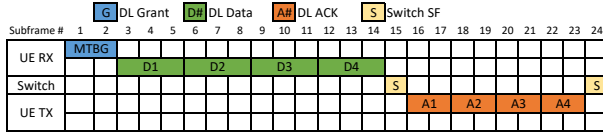
Fig. 5. Timing diagram for downlink operation with MTBG at the UE-end. UE: user equipment; RX: reception; TX: transmission; MTBG is the multiple transport block grant scheduling the downlink data D1, D2, D3, and D4, respectively. D1, D2, D3, and D4 are each repeated three times and therefore span three subframes each. A1, A2, A3, and A4 are the acknowledgment subframes of D1, D2, D3, and D4, respectively. A1, A2, A3, and A4 are each repeated two times and hence span two subframes each. S represents a switching subframe.
