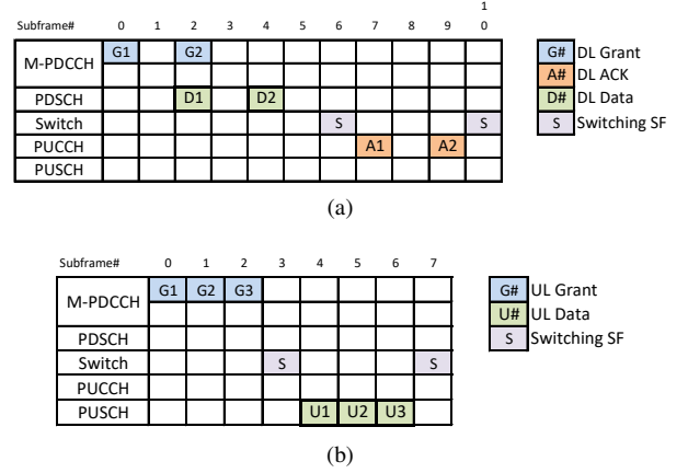
Fig. 2. Timing diagrams for LTE-M operation in (a) the downlink and (b) the uplink. M-PDCCH: machine-type communication physical downlink control channel; PDSCH: physical downlink shared channel; PUCCH: physical uplink control channel; PUSCH: physical uplink shared channel. In (a), G1 and G2 are the downlink grants scheduling the downlink data D1 and D2, respectively, and A1 and A2 are acknowledgment subframes of D1 and D2, respectively. In (b), G1, G2, G3 are the uplink grants scheduling the uplink data U1, U2, and U3, respectively. S represents a switching subframe in both sub-figures.
