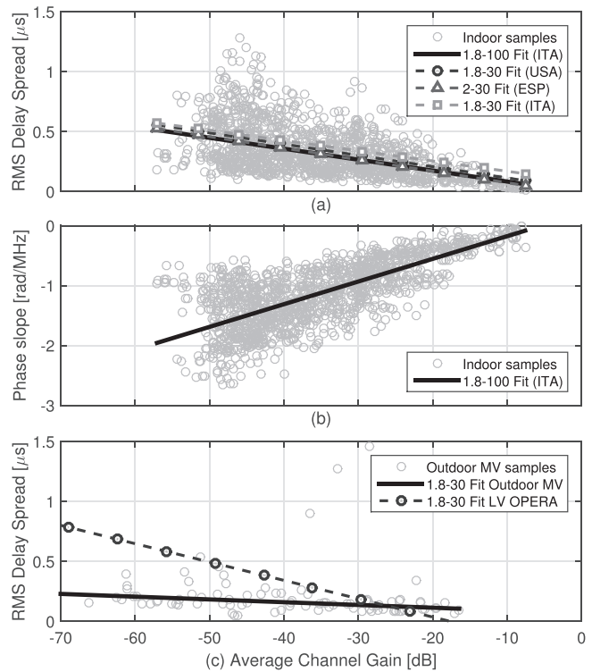
Fig. 4. RMS-DS versus ACG for the in-home scenario in the 1.8–100 MHz band (a) and the outdoor MV scenario in the 1.8–30 MHz band (c), with the corresponding robust regression fit. The robust fits for the 2–30 MHz Spanish (ESP) [64], 1.8–30 MHz USA [65] and our (ITA) 1.8–30 MHz measurements (a), and the 1.8–30 MHz LV OPERA [66] model (c) are also shown. The unwrapped phase slope versus ACG for the in-home scenario, together with the robust fit, are reported in (b).
