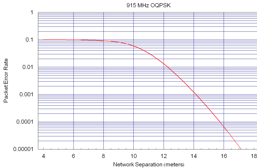
Figure E.14—Coexistence methodology results for 915 MHz O-QPSK PHY
