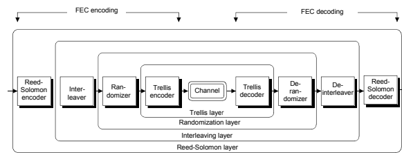
Figure B.7 – Layers of processing in the FEC
