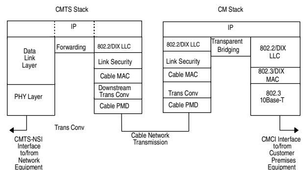
Figure 3-2. Data Forwarding Through the CM and CMTS
