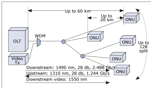
Figure 1. G-PON physical network architecture.
