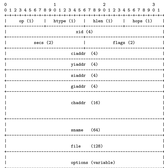
Figure 1: Format of a DHCP message
