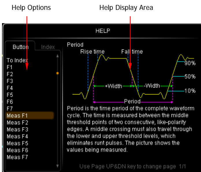
Figure 13 Help Information
