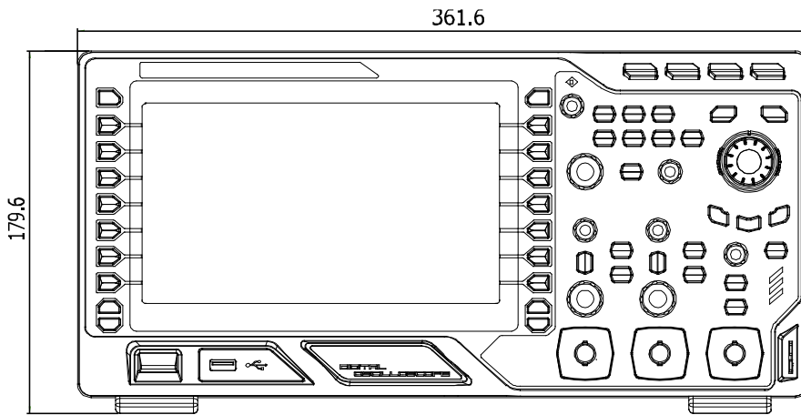
Figure 1 Front View
