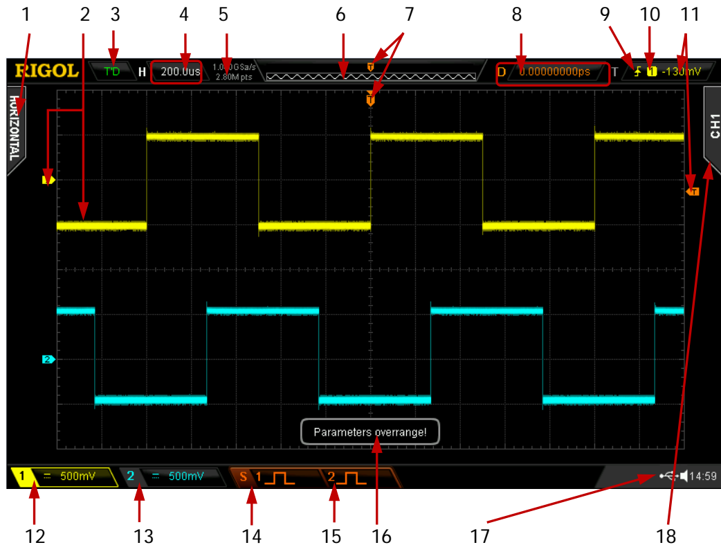
Figure 11 User Interface
