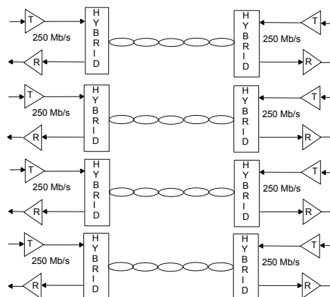
Figure 40-2—1000BASE-T topology
