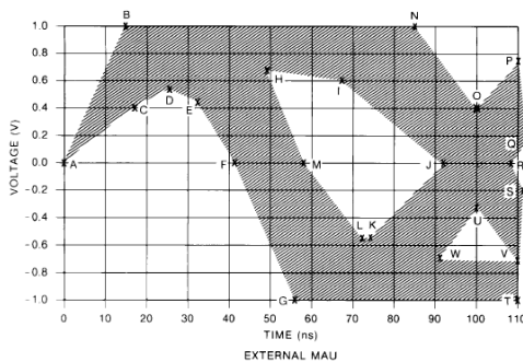
Figure 14-10—Voltage template
