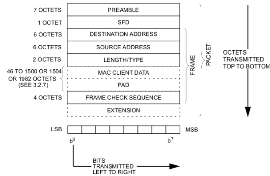
Figure 3-1—Packet format
