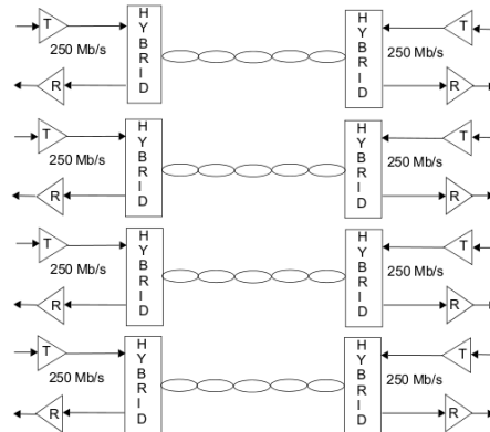
Figure 40-2—1000BASE-T topology
