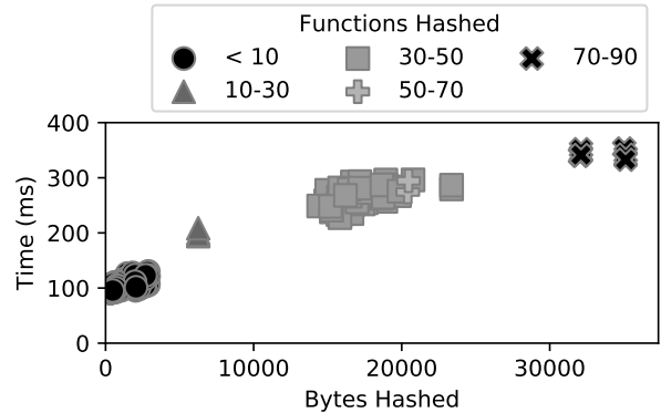
Fig. 4. Overall time to hash Java and Scala functions from our resilience benchmark using the UDF hashing library.
