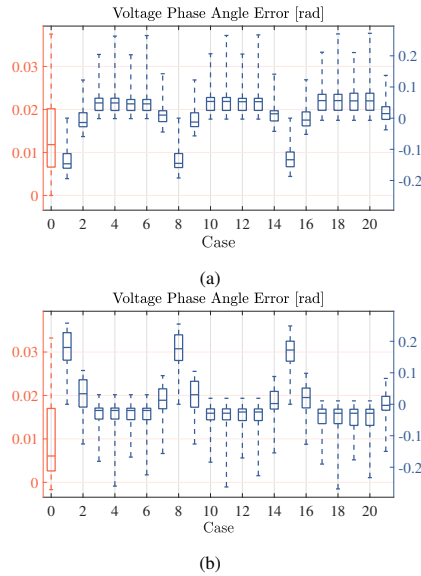
Fig. 5: Distribution of errors in phase angles from DC power flow for scenarios of uniform load change of +10% in (a) and –10% in (b). Case 0 corresponds to the distributed slack bus formulation, while Cases 1–21 are exhaustive combinations of single slack bus choices (detailed in Table II). The y axes on the left apply to Case 0, while the ones on the right apply to Cases 1–21.
