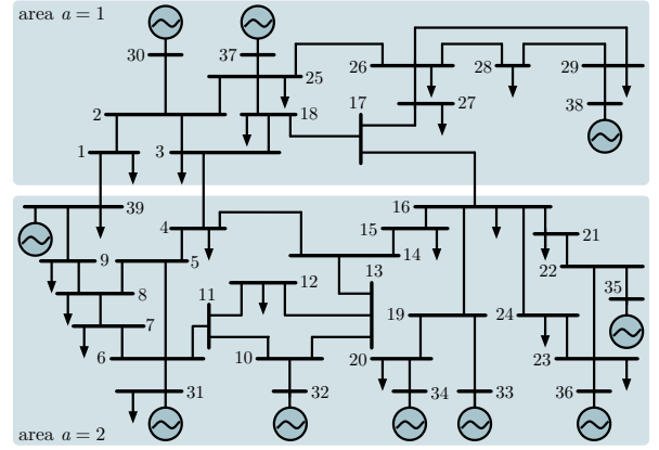
Fig. 3: One-line diagram for the New England test system.
