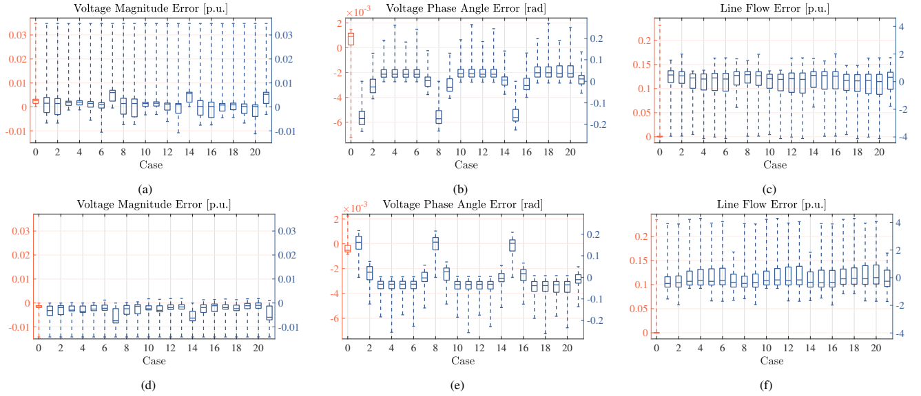
Fig. 4: Distribution of errors in (a)(d) voltage magnitudes, (b)(e) voltage phase angles, and (c)(f) line active-power flows, from AC power flow, for scenarios of uniform load change of +10% in (a)–(c) and –10% in (d)–(f). Case 0 corresponds to the distributed slack bus formulation, while Cases 1–21 are exhaustive combinations of single slack bus choices (detailed in Table II). The y axes on the left apply to Case 0, while the ones on the right apply to Cases 1–21.
