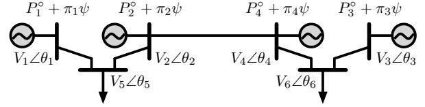
Fig. 1: Generator active-power injections are modeled as P_g^o + \pi_g\psi in the distributed slack bus formulation. This paper uncovers appropriate values for P_g^o , \pi_g , and \psi , so that bus voltage magnitudes and phase angles solved from the power flow match steady-state results from a dynamic simulation.
