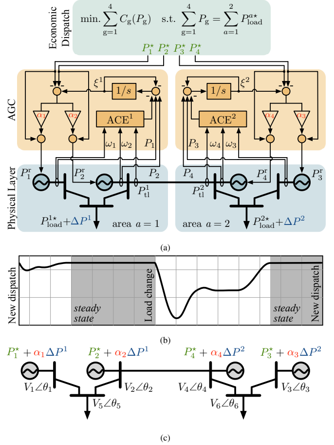
Fig. 2: (a) Illustration of economic dispatch and AGC architecture for a power system with two control areas. (b) [not to scale] Sketch of prevailing frequency in a control area. Steady-state operation (shaded gray) is punctuated by dynamic excursions that may arise due to new economic dispatch setpoints or load changes. (c) Power flow formulation with distributed slack bus. Modeling injections of generator buses as P_g^* + \alpha_g \Delta P^a in the algebraic power flow equations yields the best estimates for bus voltage magnitudes and phase angles during periods of steady state between economic dispatch updates.
