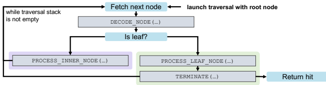
Fig. 2: Abstraction of the tree traversal algorithm
