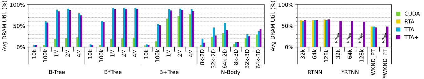
Fig. 13: DRAM utilization of selected applications on the non-accelerated baseline GPU, baseline RTA, TTA, and TTA+
