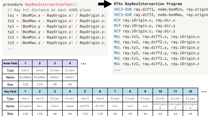
Fig. 11: Example of TTA+ intersection test
