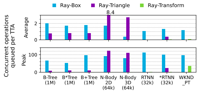
Fig. 15: TTA Intersection unit utilization for sample applications. (*WKND_PT is not supported by TTA)
