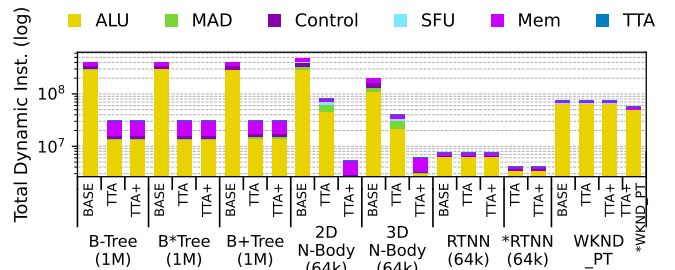
Fig. 20: Breakdown of total dynamically executed instructions for baseline, TTA, and TTA+
