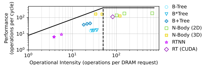
Fig. 6: GPU roofline model for tree traversal applications
