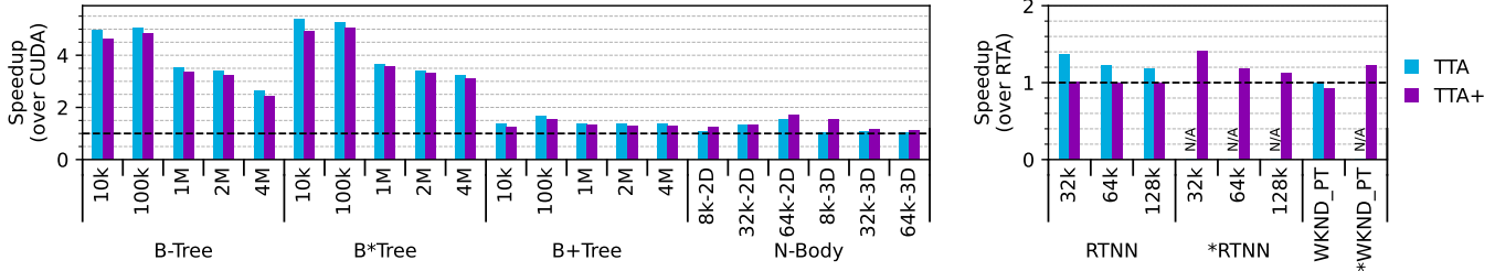
Fig. 12: Performance of selected applications on TTA and TTA+ relative to baseline GPU (CUDA applications – left, RTA applications – right)
