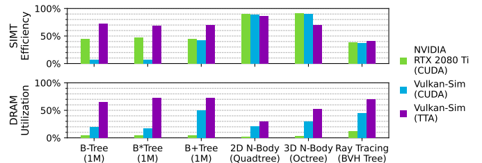
Fig. 1: SIMT efficiency and DRAM bandwidth utilization of tree traversal applications on GPUs with and without TTAs.
