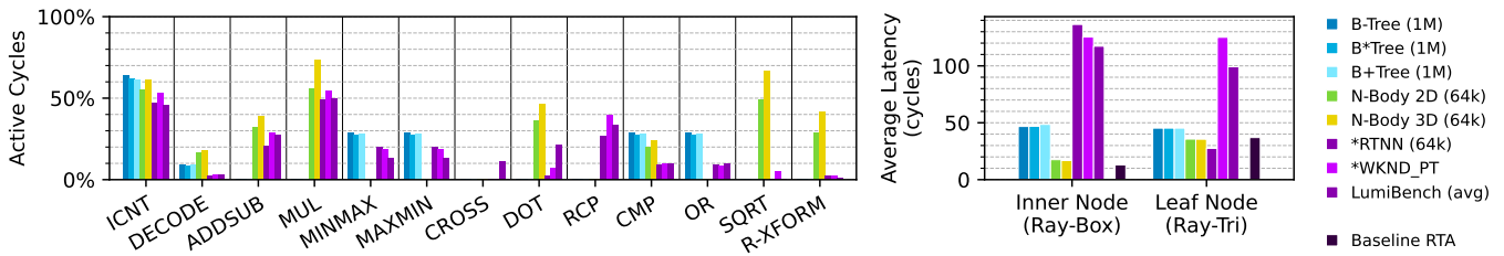
Fig. 18: OP unit utilization (left) and average intersection latency (right) for applications on TTA+
