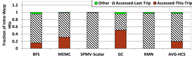
Figure 4: Classification of intra-warp hits within loops using an 8M L1D cache. Accessed-This-Trip=hit on data already accessed this loop iteration. Accessed-Last-Trip=hit on data accessed in immediately-previous loop iteration.
