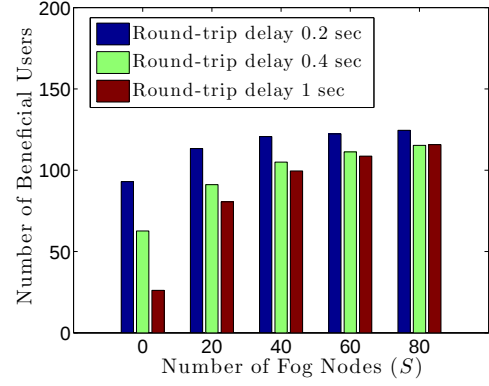
Fig. 6. The number of users that find the computing services beneficial and offload their tasks affected by the roundtrip delay. The QoE of these users are greater than zero ( N = 200 ).
