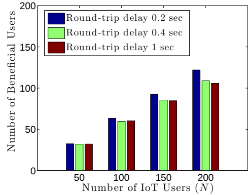
Fig. 7. The number of beneficial users affected by the roundtrip delay when S = 50 .
