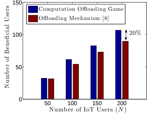
Fig. 10. The number of beneficial users versus the number of IoT users. Our proposed mechanism outperforms the offloading mechanism proposed in [8] by up to 20 % in terms of the number of beneficial users ( S = 60 ).
