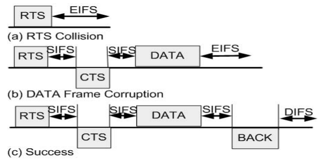
Fig. 3. Uni-directional RTS/CTS Access Scheme.
