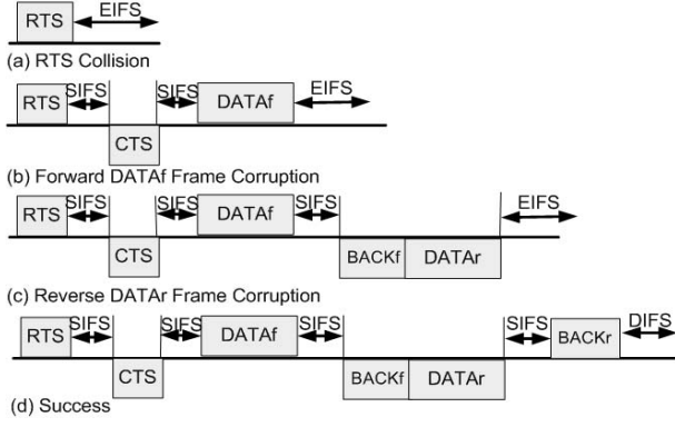
Fig. 4. Bi-directional RTS/CTS Access Scheme.
