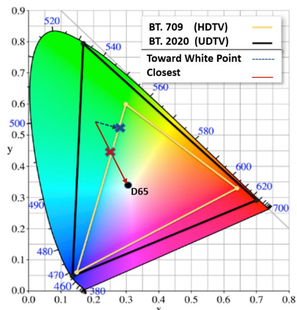
Fig. 1. CIE 1921 xy chromaticity diagram with the BT.709 and BT.2020 color gamuts, arrows illustrate Toward White point (TWP) and Closest projection techniques.
