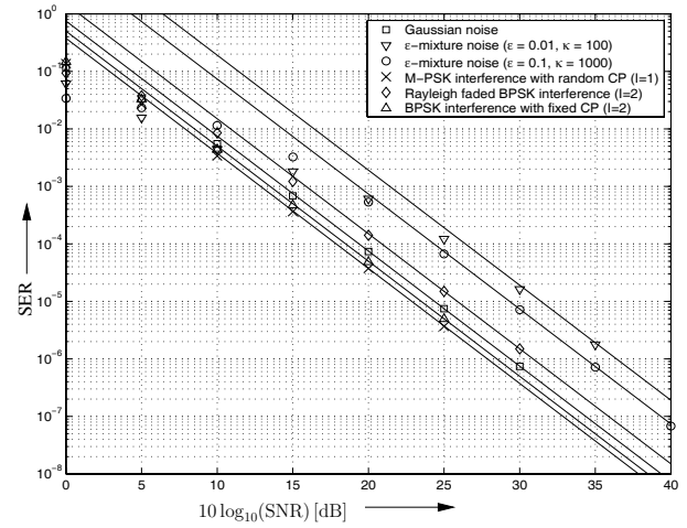
Fig. 2. SER vs. SNR for BPSK over a Nakagami- m fading channel with m = 2 and different types of noise discussed in Sections II-C, II-D. \epsilon -mixture noise: Example E1) in Section II-C. M -PSK interference with random channel phase (CP): Example E3) in Section II-C. Rayleigh faded BPSK interference: Example E5) in Section II-D. BPSK interference with fixed CP: Example E2) in Section II-C. Markers: Simulated SER. Solid lines: Asymptotic SER [Eq. (18)].
