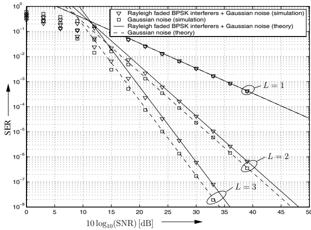
Fig. 5. SER vs. SNR per branch for 8-PSK over a Rayleigh fading channel with EGC. All diversity paths have the same average SNR. Markers: Simulated SER. Solid lines: Asymptotic SER for Rayleigh faded BPSK interference (two interferers) and Gaussian noise [Eq. (29)]. Dashed lines: Asymptotic SER for Gaussian noise [Eq. (29)].
