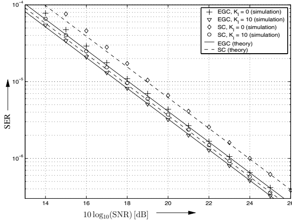
Fig. 4. SER vs. SNR per branch for BPSK over a Ricean fading channel with Ricean factor K = 2 , L = 2 diversity branches, and Ricean faded M -PSK interference. The interference channel has Ricean factors of K_I = 0 and K_I = 10 , respectively. All diversity paths have the same average SNR. EGC and SC are considered. Markers: Simulated SER. Solid lines: Asymptotic SER for EGC [Eq. (29)]. Dashed lines: Asymptotic SER for SC [Eq. (33)].
