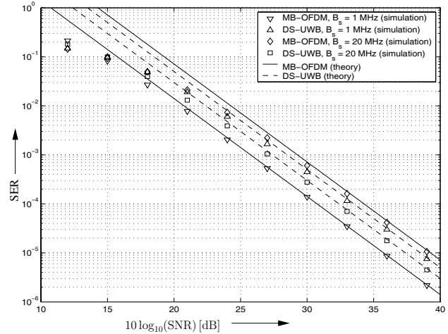
Fig. 3. SER vs. SNR for 16-QAM with bandwidth B_s over a Nakagami- m fading channel with m = 2 and UWB interference. Markers: Simulated SER. Solid lines: Asymptotic SER for MB-OFDM interference [Eq. (18)]. Dashed lines: Asymptotic SER for DS-UWB interference [Eq. (18)].
