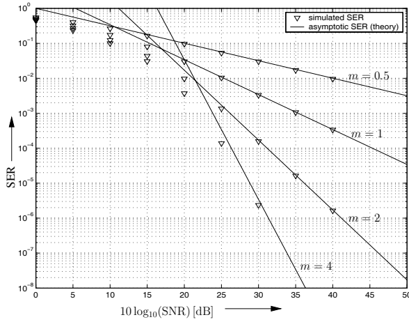
Fig. 1. SER vs. SNR for 8-PSK over a Nakagami- m fading channel with \epsilon -mixture noise ( \epsilon = 0.25 , \kappa = 10 ). Markers: Simulated SER. Solid lines: Asymptotic SER [Eq. (18)].
