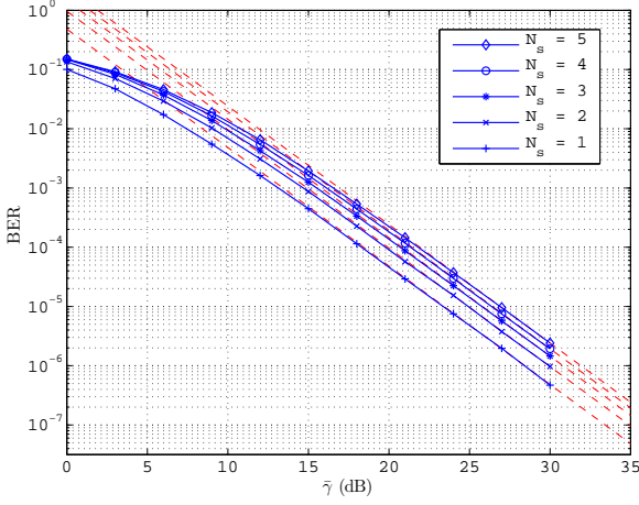
Fig. 2. Average BER vs. SNR \bar{\gamma} of an NCCD system with N_s sources and BPSK. Solid lines with markers: Simulated BER. Dashed lines: Asymptotic BER [(20), (26)].
