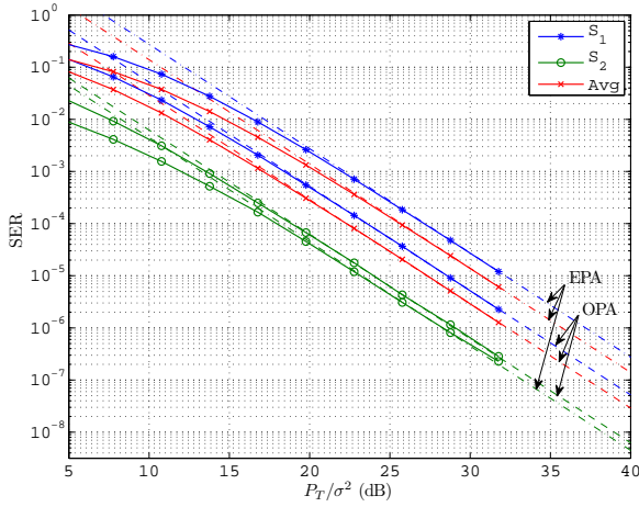
Fig. 3. SER vs. P_T/\sigma^2 of an NCCD system with 8-PSK for OPA and EPA. Solid lines with markers: Simulated SER. Dashed lines: Asymptotic SER [(20)].
