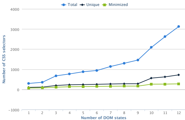
Figure 13: Rate of Convergence of DOM element locators for Facebook.
