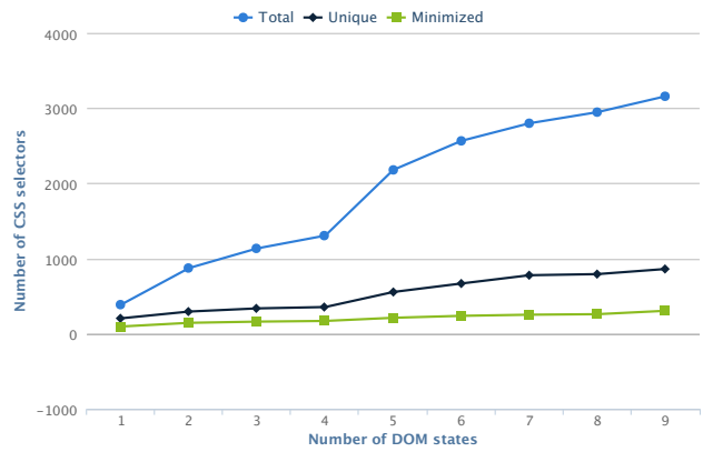
Figure 14: Rate of Convergence of DOM element locators for Wikipedia.
