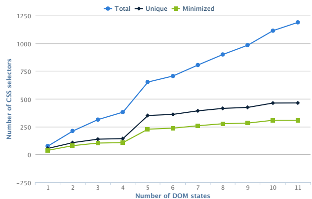
Figure 15: Rate of Convergence of DOM element locators for Bing Search Engine.
