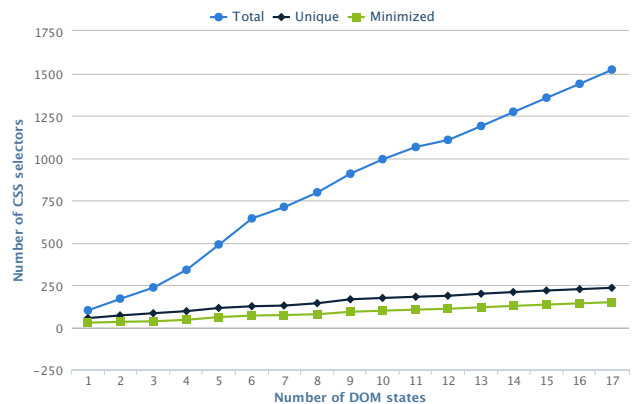
Figure 16: Rate of Convergence of DOM element locators for a Wordpress based blog.
