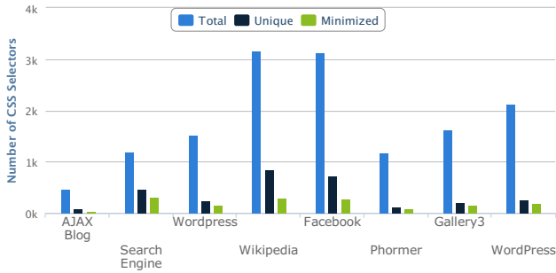
Figure 8: Convergence of DOM element locators for different websites.
