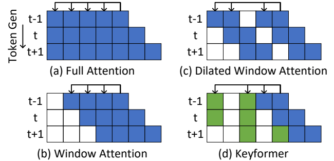
Figure 2. Attention block for generative inference. (a) Full attention (Brown et al., 2020) with current token attending all previous tokens. (b) Window attention ( w = 4 ): Focusing on the most recent 4 tokens. (c) Dilated window attention ( w = 4 , dilation = 1). (d) Keyformer ( w = 2 , k = 2 ): A mix of recent window ( w ) and key tokens ( k ). White color indicates no attention, while blue color indicates attention. The green color identifies the key tokens and their respective attention. The values of the three consecutive token generation iterations are t - 1, t, t + 1 .
