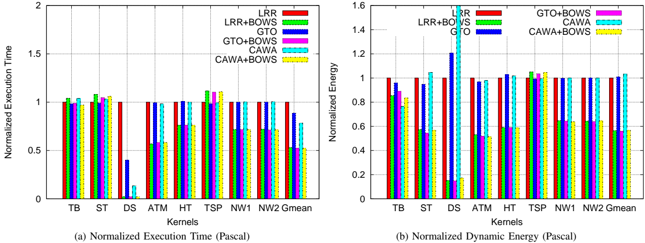
Figure 15: Performance and Energy Savings on Pascal
