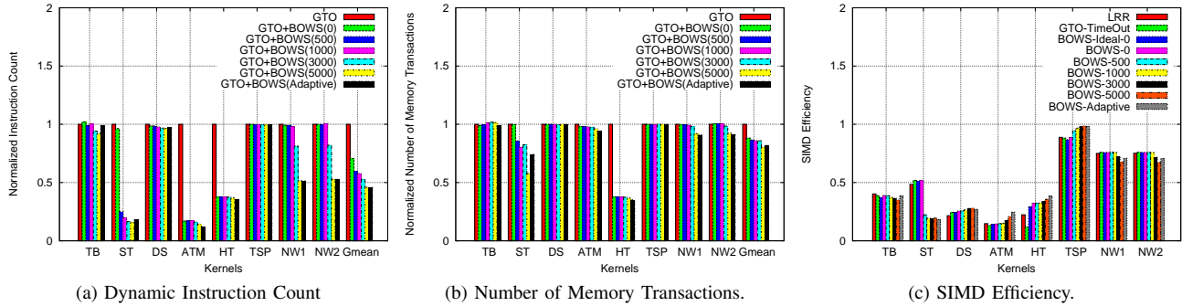
Figure 13: BOWS Impact on Dynamic Overheads.
