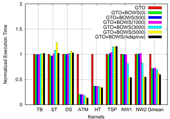
Figure 10: Normalized Execution Time at Different Back-off Delay Limit Values (using DDOS).
