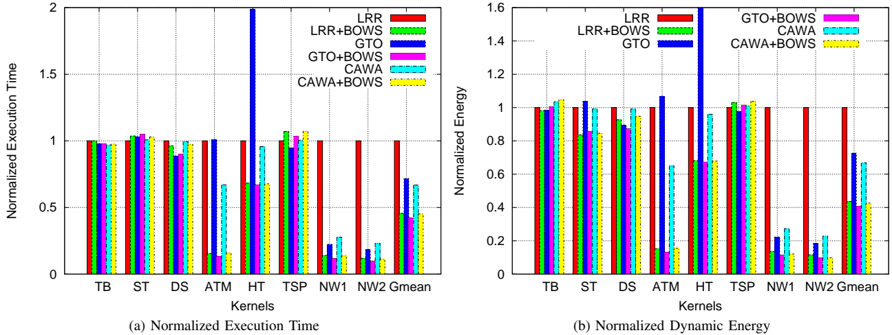
Figure 9: Performance and Energy Savings on GTX480 (Fermi)
