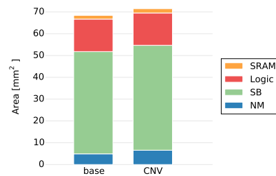
Fig. 11: Area Breakdown
