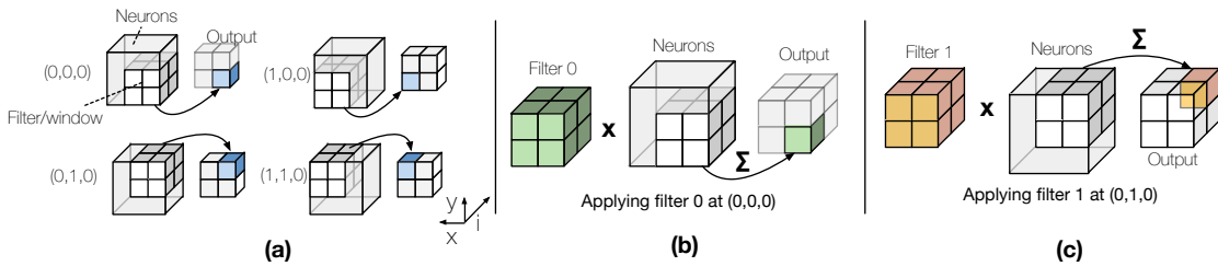
Fig. 2: The output neuron at position (0, 0, 0) or o(0, 0, 0) is produced by applying the filter on a 2 \times 2 \times 2 window of the input with origin n(0, 0, 0) . Each synapse s(x, y, z) is multiplied by the corresponding input neuron n(x, y, z) , e.g., n(0, 0, 0) \times s(0, 0, 0) , and n(0, 1, 0) \times s(0, 1, 0) , for a total of 2 \times 2 \times 2 or eight products. The eight products are reduced into a single output neuron using addition. Then the window is slide over by S first along the X dimension to produce o(1, 0, 0) using the neuron input window at origin n(1, 0, 0) . For example, now s(0, 0, 0) is multiplied with n(1, 0, 0) and s(1, 1, 0) with n(2, 1, 0) . Once the first dimension is exhausted, then the window slides by S along the Y dimension and starts scanning along the X dimension again, and so on as the figure shows. In total, the result is a 2 \times 2 \times 1 output neuron. The depth is one since there is only one filter. Parts (b) and (c) show a convolutional layer with two 2 \times 2 \times 2 filters. The output now is a 2 \times 2 \times 2 array, with each filter producing one of the two planes or layers of the output. As part (b) shows, the first filter produces output elements o(x, y, 0) . Part (c) shows that the second filter produces output neurons o(x, y, 1) .
