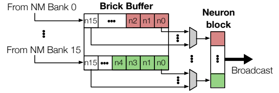
Fig. 8: Dispatcher
